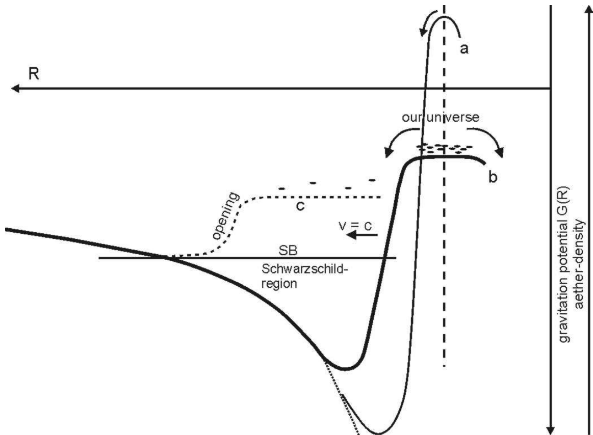
Fig. 2: Purely schematic presentation of the radial gravitation potential G(R) or aether density of 'our universe' in the 'early past' (a), at present (b) and for a future state of 'opening' (c). According to the extreme ratio in the dimension of inner and outer regions, as well the axes as the relations to each other are given only exemplary and distorted (the central region strongly enlarged). The vertical dashed line gives the position of the Big Bang. The outermost left graph (dotted in the lower part) represents the gravitation-funnel at the moment of Big Bang.
