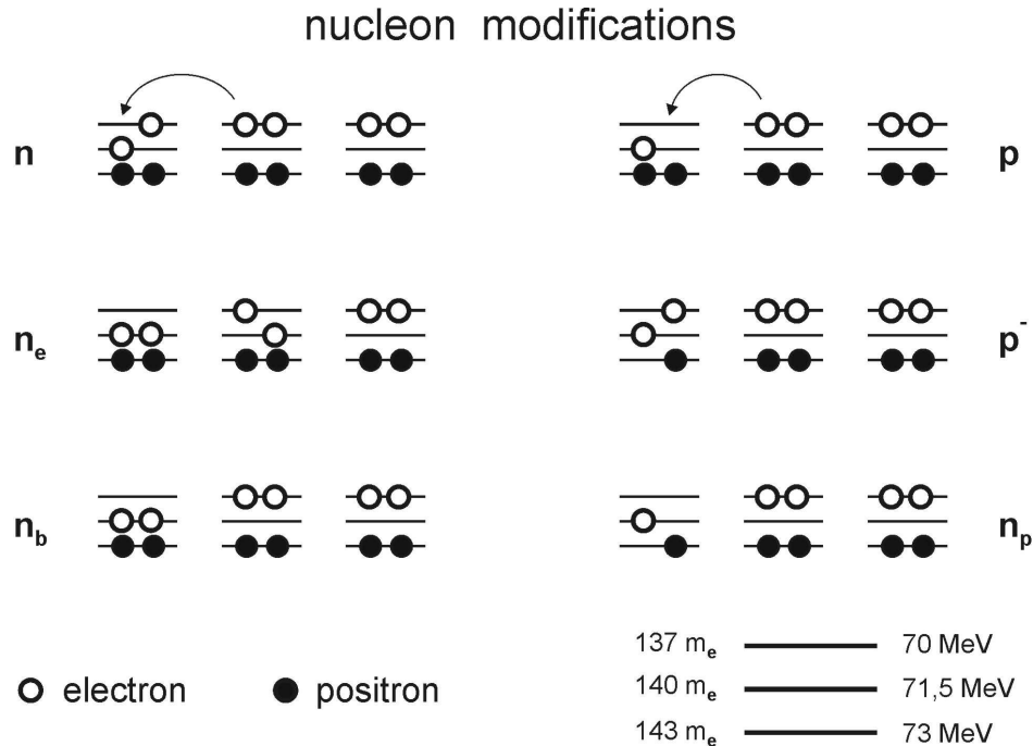
Fig. 1: Scheme of occupation states of the lepton orbitals of the three Quarks (without spin orientations) within different kinds of nucleons. In the lower right the corresponding lepton energies within the sub-orbitals of the three Quarks are given. The cyclic exchange processes of the relativistic electrons (Strong Interaction) are symbolised by arrows. The middle orbital is occupied by leptons without electron-neutrino coupling. There are two further thinkable non-documented neutrino-depleted neutron modifications (one of it bosonic).
